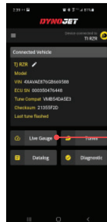
Live Gauge
