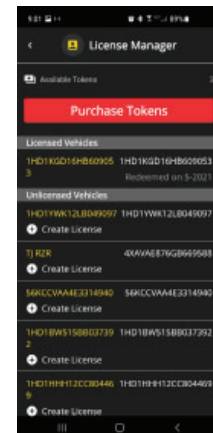
License Manager
