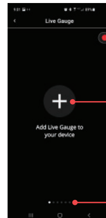
Live Gauge
