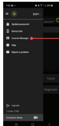
License Manager
