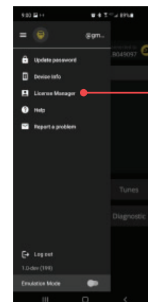
License Manager
